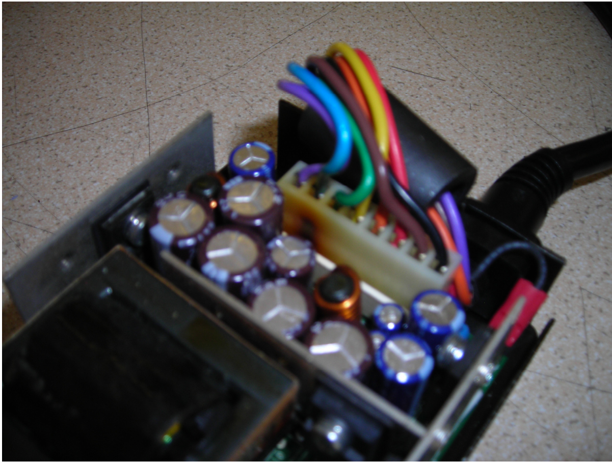
Burned Connector. This was present before the total failure.
